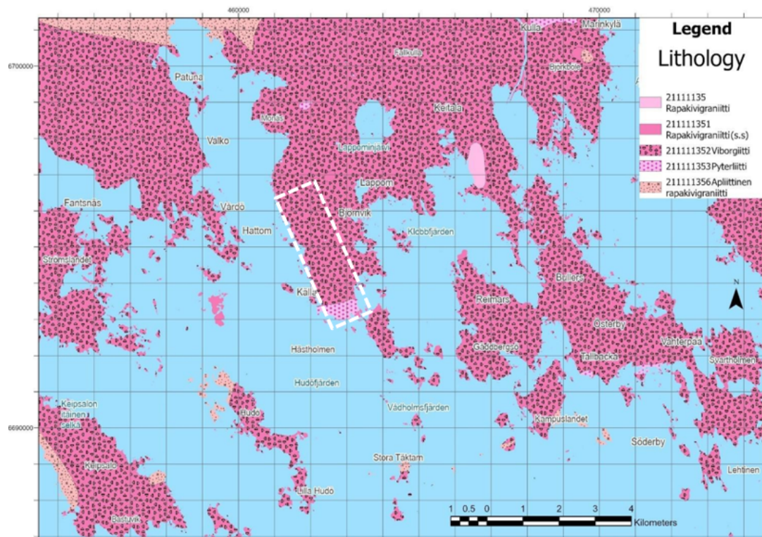
Figure 2. Lithological map of the Källa planning area and its surrounding areas. The area under consideration is indicatively outlined by a white dotted line. Lithological = description of a rock based on its physical features.
