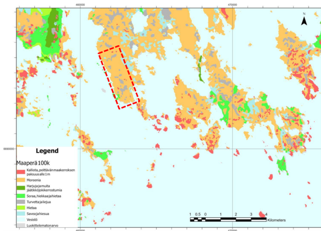
Figure 1. Soil map in the Källa planning area and its surrounding areas. The area under review is indicatively outlined by a red dotted line.
